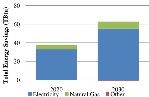
Figure 7: Residential Sector Savings by Fuel Type
